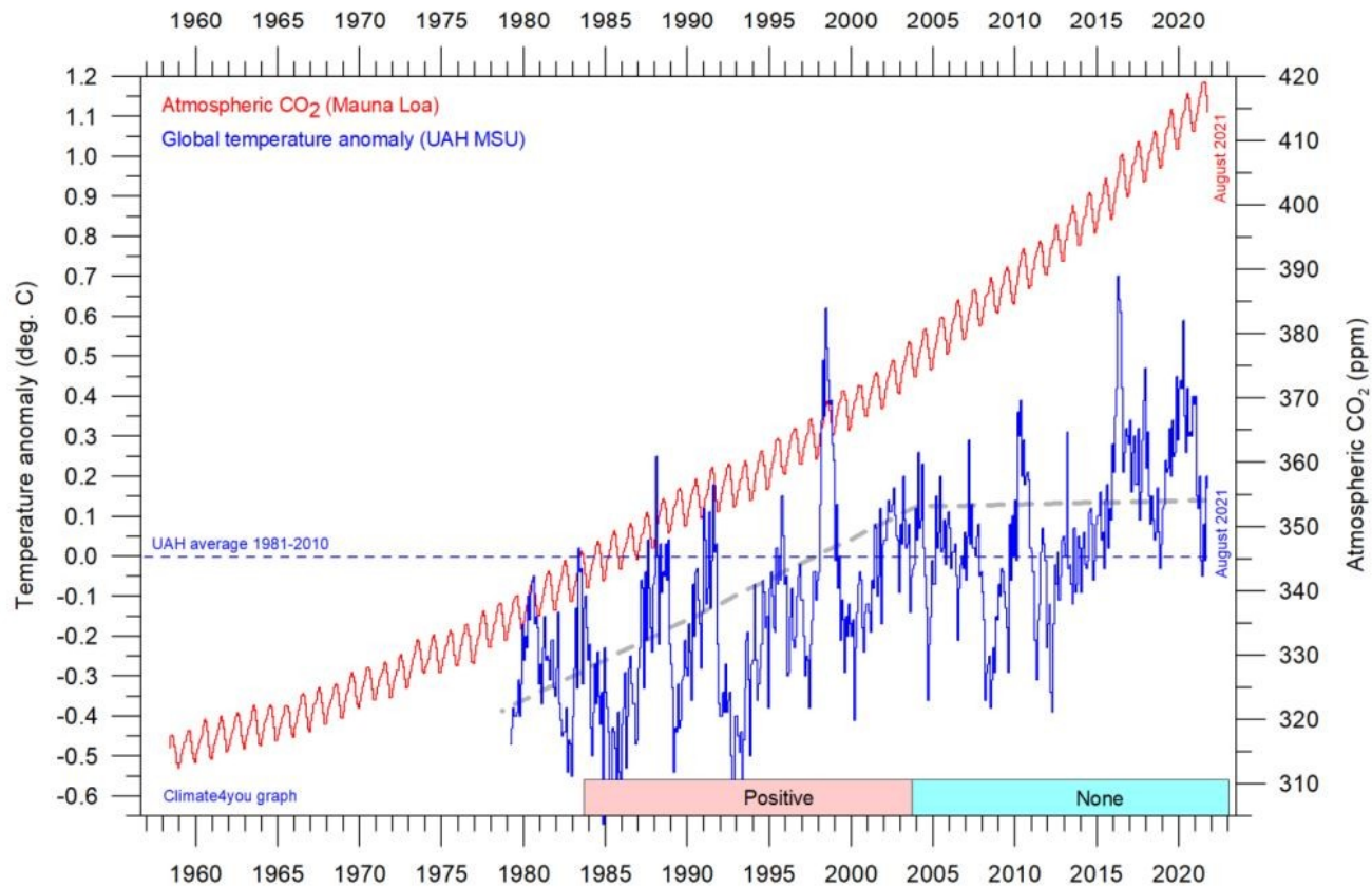
Global air temperature and atmospheric CO 2 , updated to August 2021
